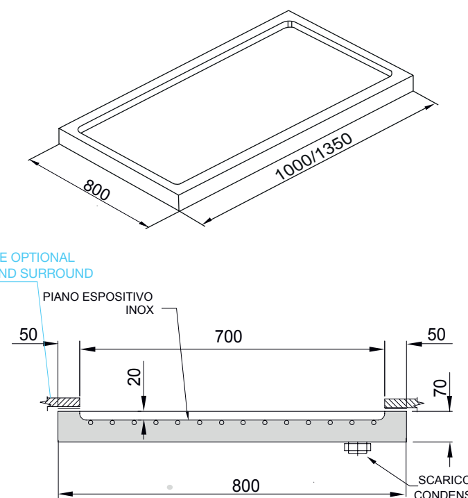
REFRIGERATA A CONTATTO EURONORM EURONORM CONTACT REFRIGERATED UNIT
