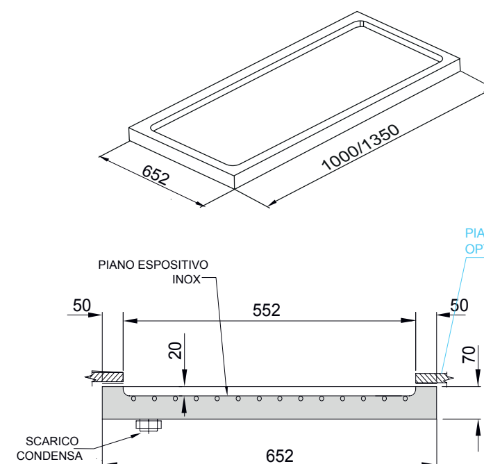
REFRIGERATA A CONTATTO GASTRONORM GASTRONORM CONTACT REFRIGERATED UNIT
